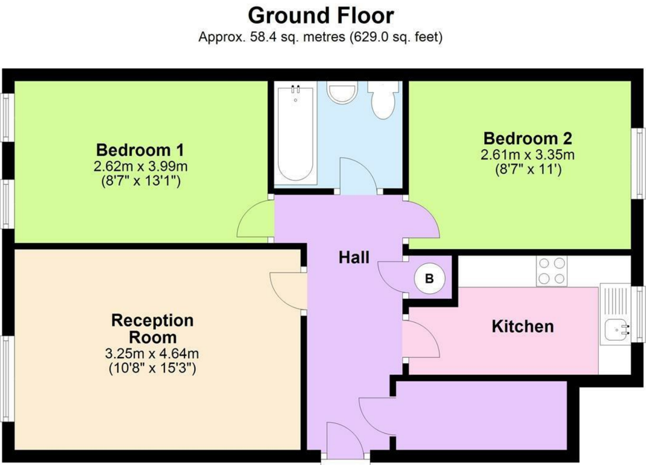
Total area: approx. 58.4 sq. metres (629.0 sq. feet) All measurements are approximate. Plan produced using PlanUp.
